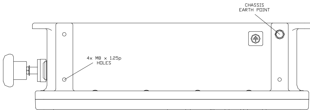
Diagram 1: Enclosure details
